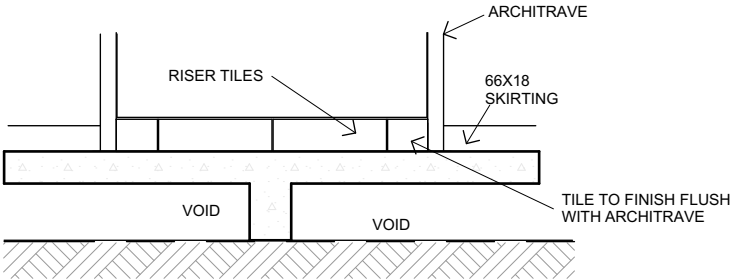
INTERNAL BEAM - HOUSE/GARAGE THRU DOOR ELEVATION A02a9
