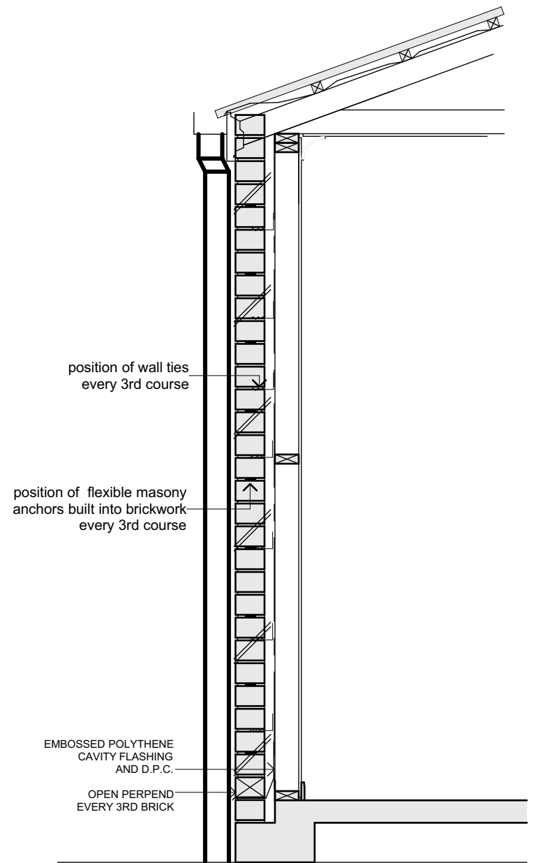
VERTICAL ARTICULATION JOINT SECTION
