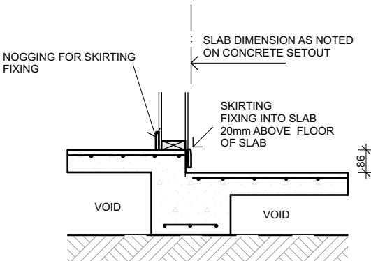
INTERNAL BEAM - HOUSE/GARAGE THRU WALL A02a5
