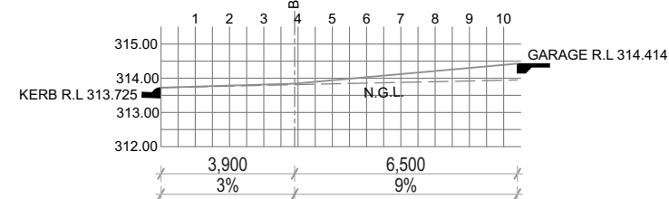
Driveway Section SCALE 1:200
