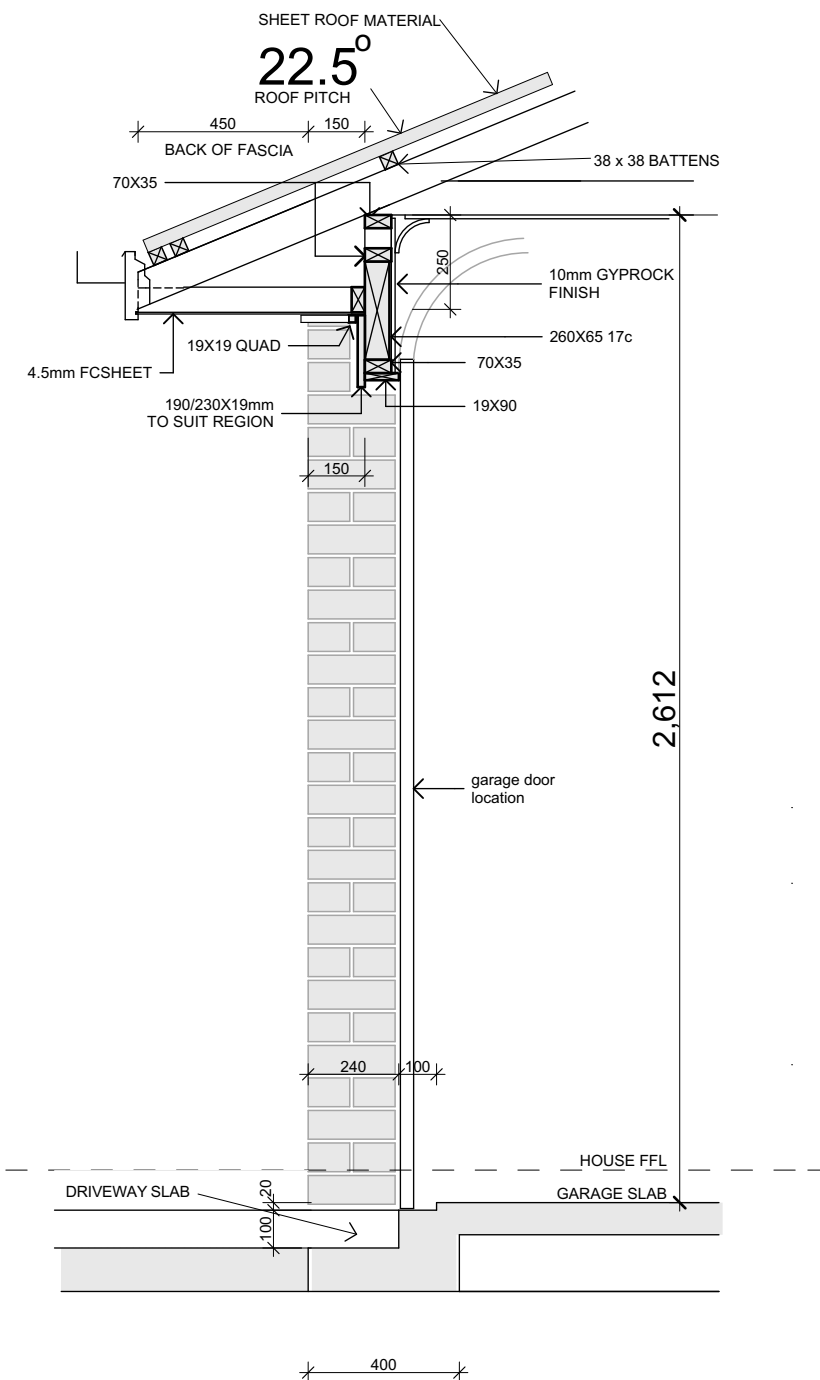
GARAGE OPENING A03
