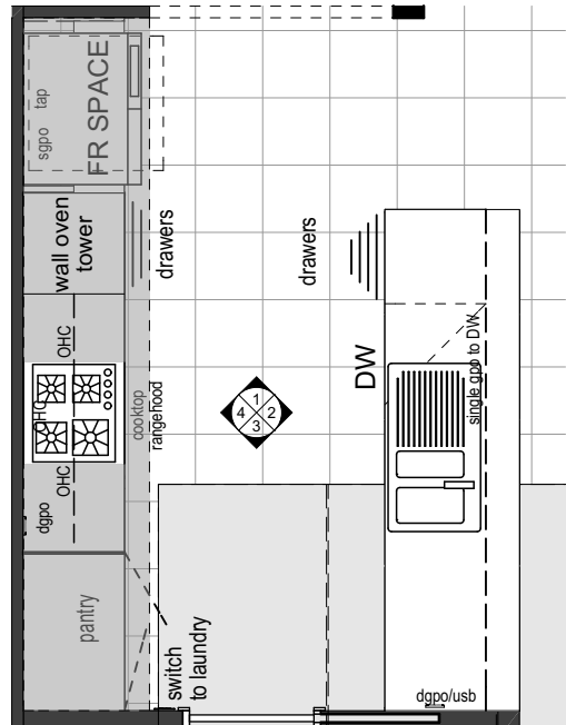
KITCHEN LAYOUT
