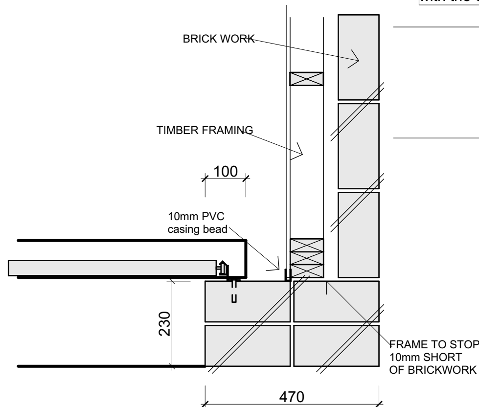
EXTERNAL CORNER A02
