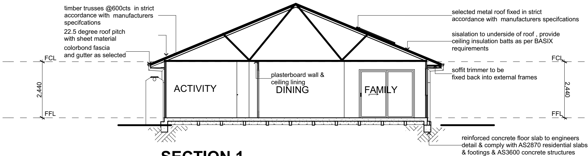
SECTION 1
