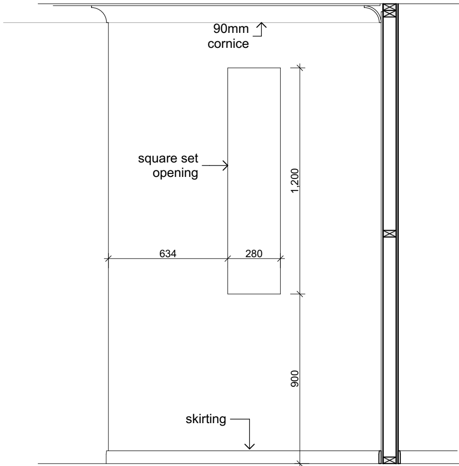
VIEW 'A' as viewed from Dining Room BETWEEN DINING & ENTRY SCALE 1:20
