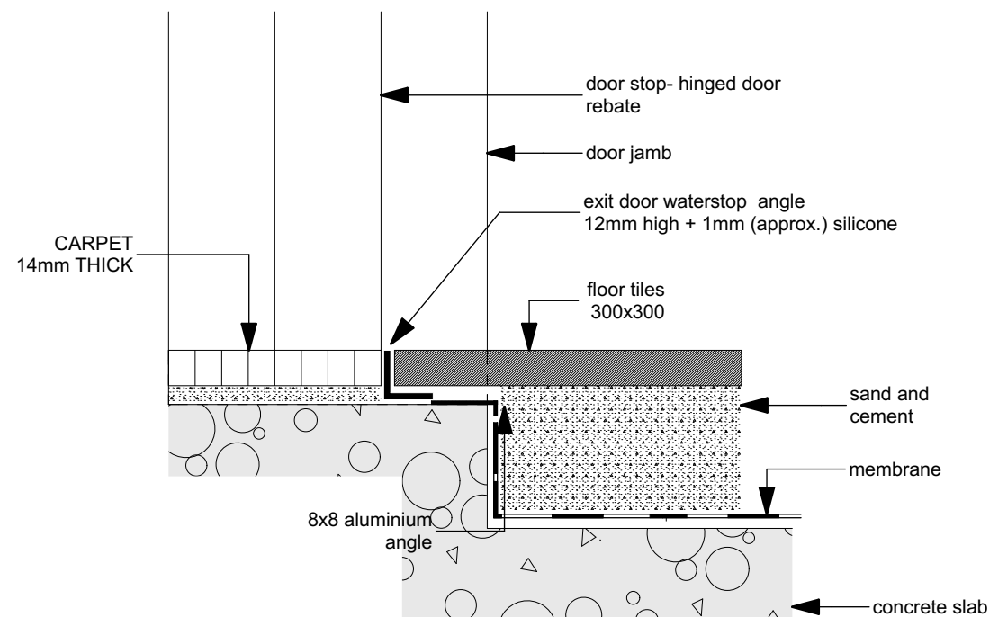
DETAIL 2
