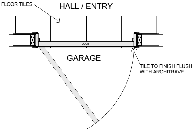
INTERNAL BEAM - HOUSE/GARAGE THRU DOOR PLAN A02a7
